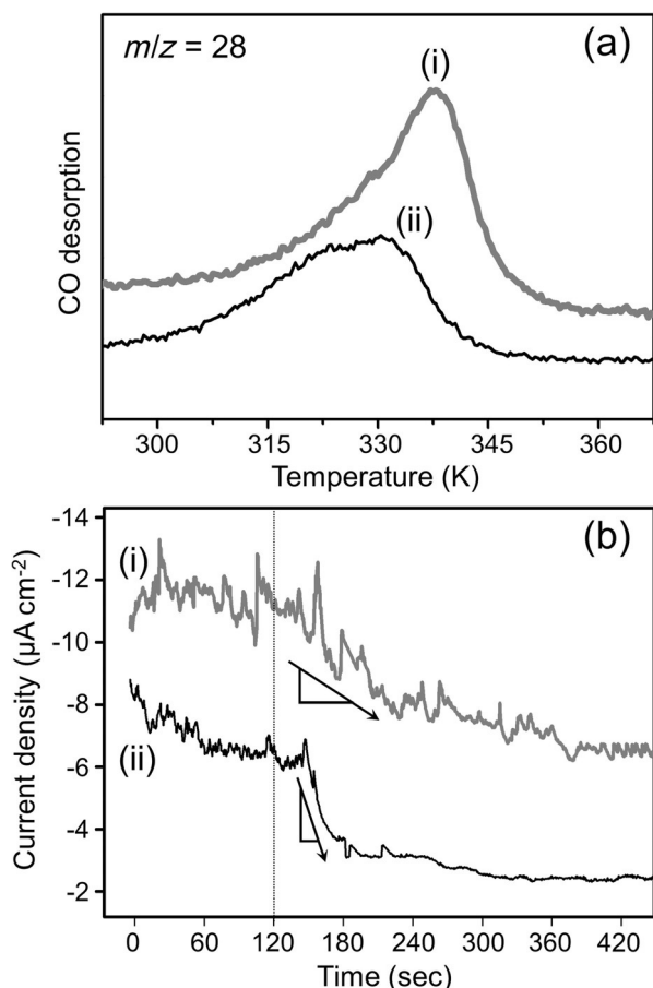
Figure 4. Experimental measurements of CO adsorption strength on the studied catalysts. a) CO TPD profiles of the (i) \text{Cu}_2\text{O}_{\text{Cl}} and (ii) \text{Cu}_2\text{O}_{\text{OE}} at ramping rate of 5 \text{ K min}^{-1} . b) Chronoamperometric measurements at constant potential of -0.32 \text{ V} (vs. RHE); i) in 0.1 M KCl and (ii) 0.1 M \text{KHCO}_3 .
